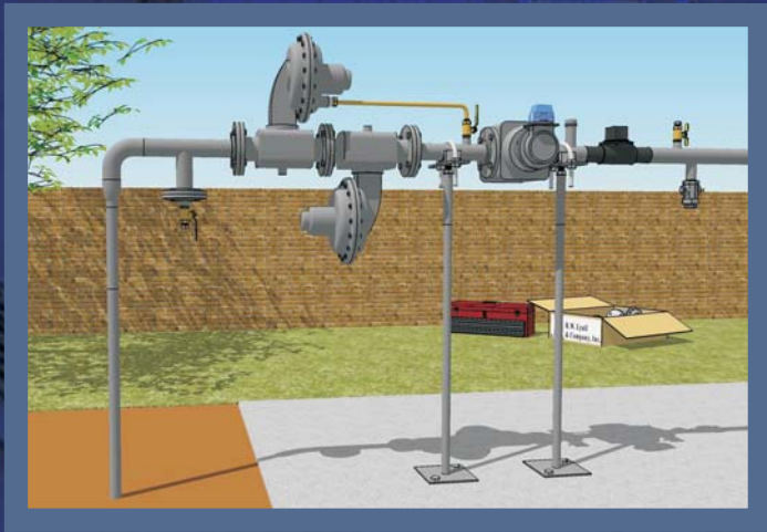
Adjustable Support Posts for Rotary Sets
